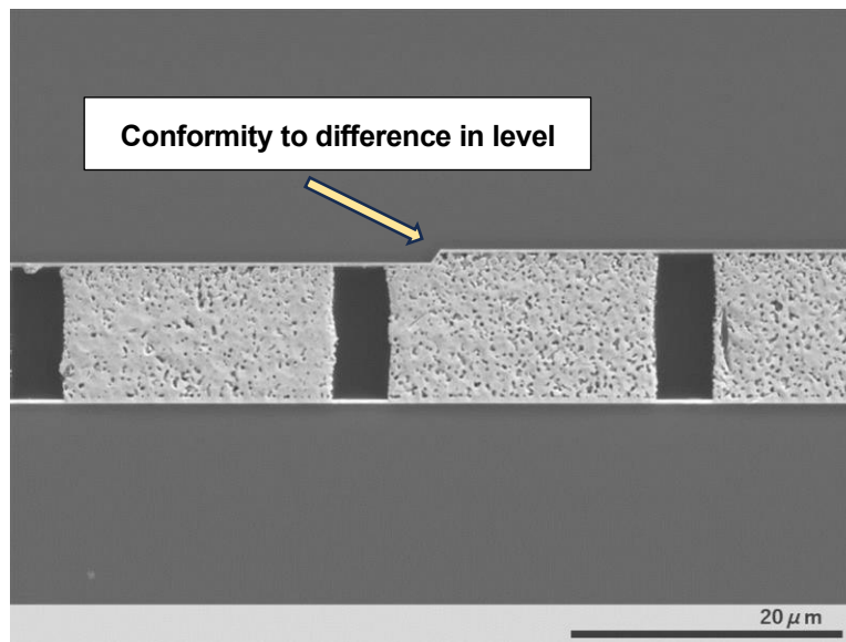
Figure 2. AuRoFUSE™ Preforms SEM image showing absorption of unevenness during bonding
