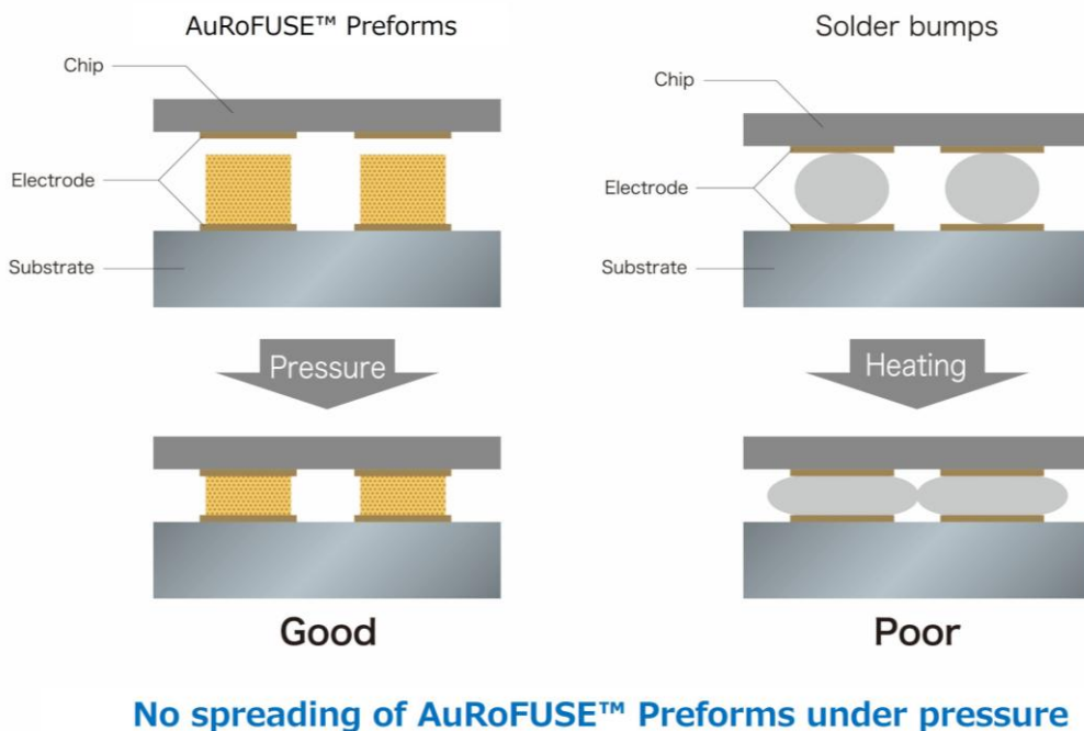
Figure 1. Comparison of AuRoFUSE™ Preforms and other materials
