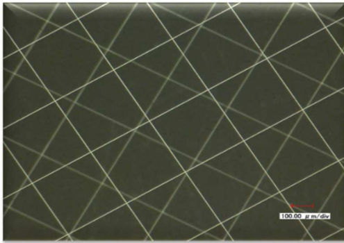
Enlarged exterior view of the metal mesh film with a single-sided, a dual-layer wiring structure for use in touch sensors
